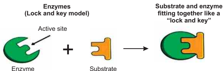
Figure 6.5 Lock and Key model
